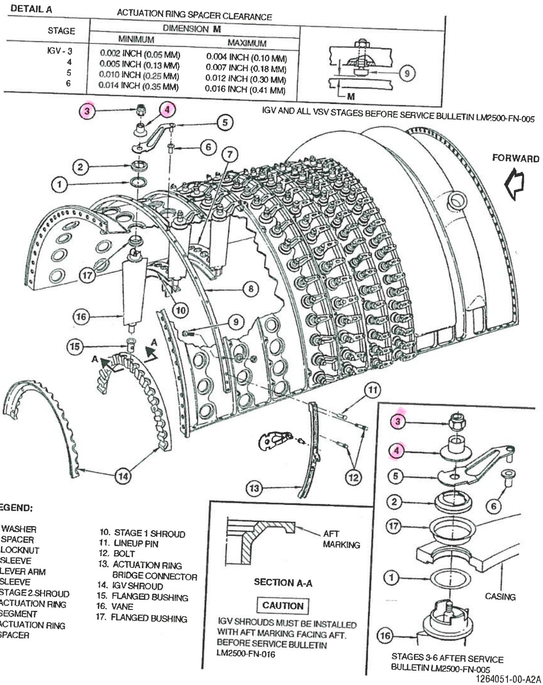
Figure 2. Assembly/Disassembly of Compressor Stator
